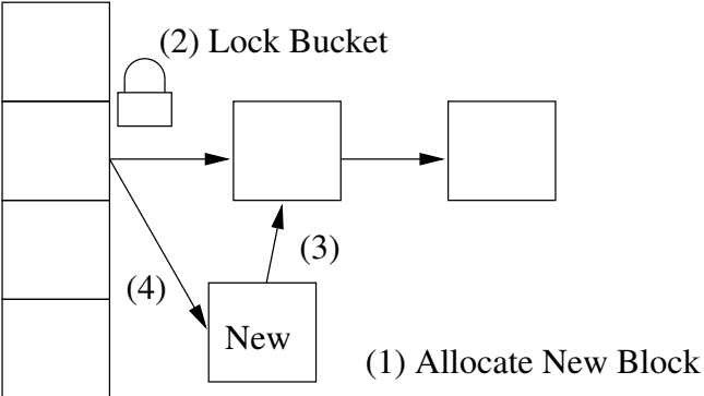
Insert Bucket Entry
