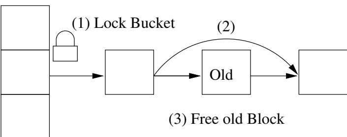
Delete Bucket Entry
