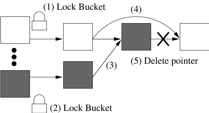
Move Entry to New Bucket
